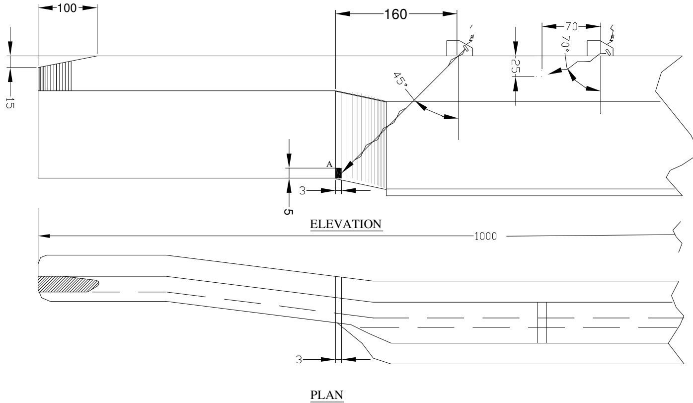
FIG. 26(c) : BEAM DIRECTION OF ANGLE PROBES FOR SENSIVITY SETTING
