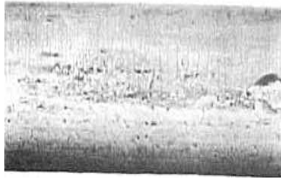
FIG. 40 : 2252 - HEAD SURFACE, WHEEL BURN REPEATED
