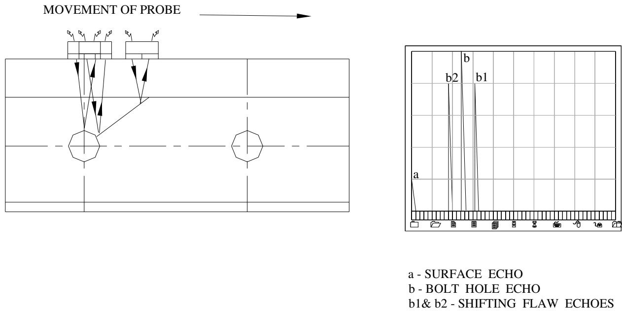
FIG. 16: BOLT HOLE WITH CRACK (TYPE 135,235,0° PROBE)
