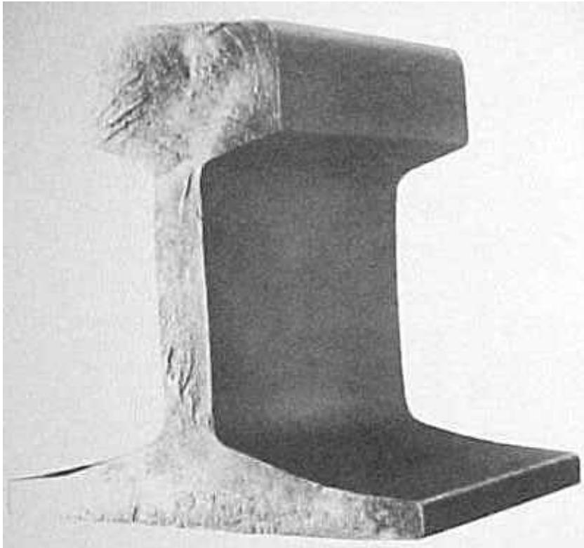
FIG. 31 : 100 OR 200 - TRANSVERSE BREAKAGE WITHOUT APPARENT ORIGIN
