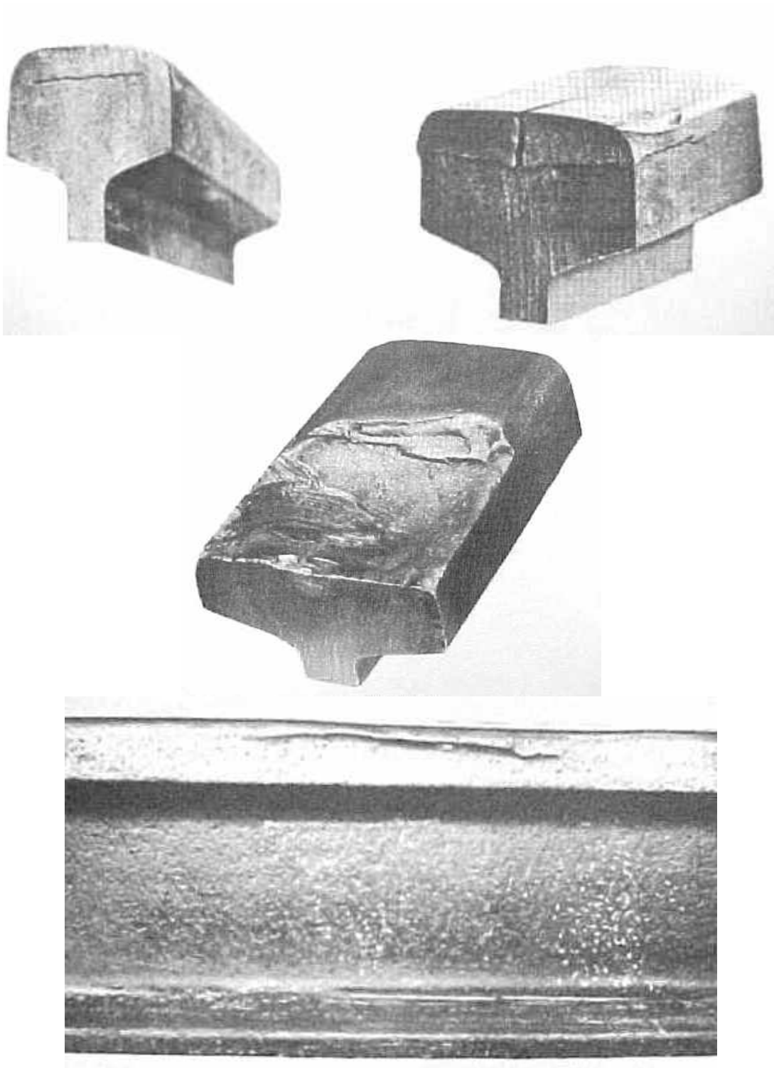
FIG. 34 : 112 OR 212 - INTERNAL FLAW IN HEAD , HORIZONTAL CRACK
