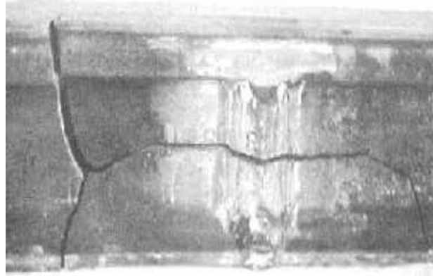
FIG. 52 : 422 - WELDING, THERMIT JOINT HORIZONTAL CRACK
