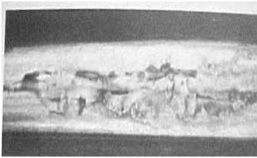
FIG. 36 : 1211 OR 2211 - HEAD, SURFACE, SHALLOW SURFACE DEFECT (FLAKING)
