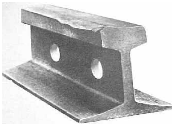
FIG. 32 : 123 OR 223 - HEAD, SURFACE CRUSHING OR BATTERING
