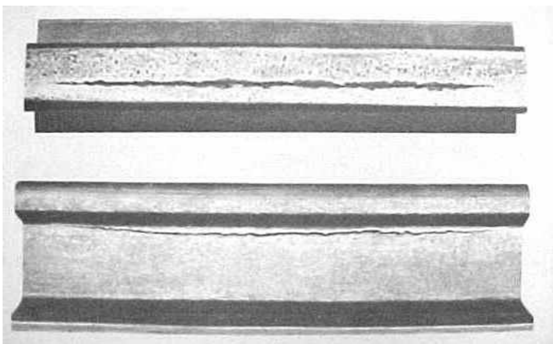
FIG. 35 : 113 OR 213 - INTERNAL FLAW IN HEAD , VERTICAL LONGITUDINAL SPLIT
