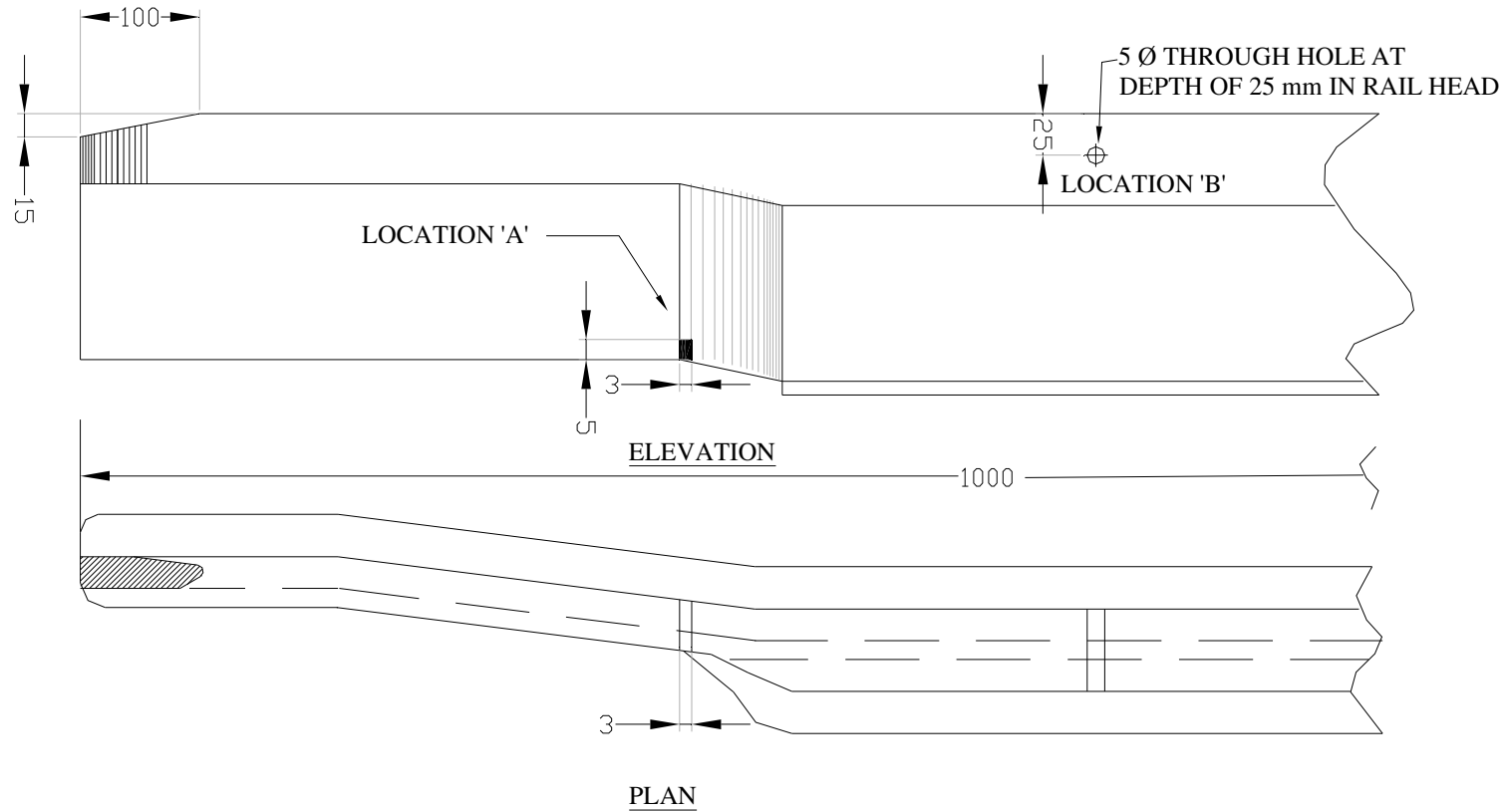
FIG. 26(b) : STANDARD TEST PIECE (SEJ STOCK RAIL)
