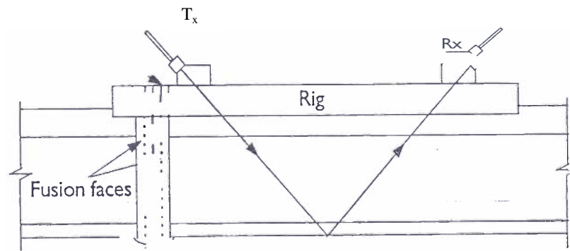
Fig.22(b): Sensitivity setting using 45^\circ tandem probe
