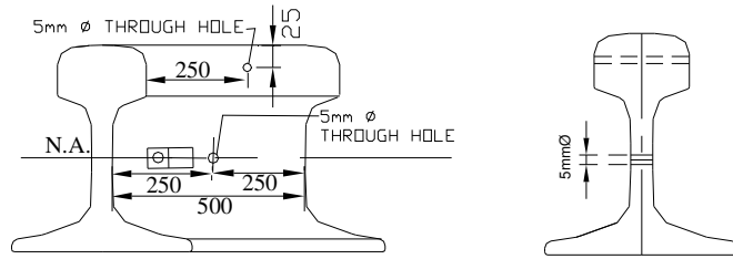
CALIBRATION AND SENSITIVITY SETTING (USING 70° PROBE) ON STANDARD RAIL PIECE
