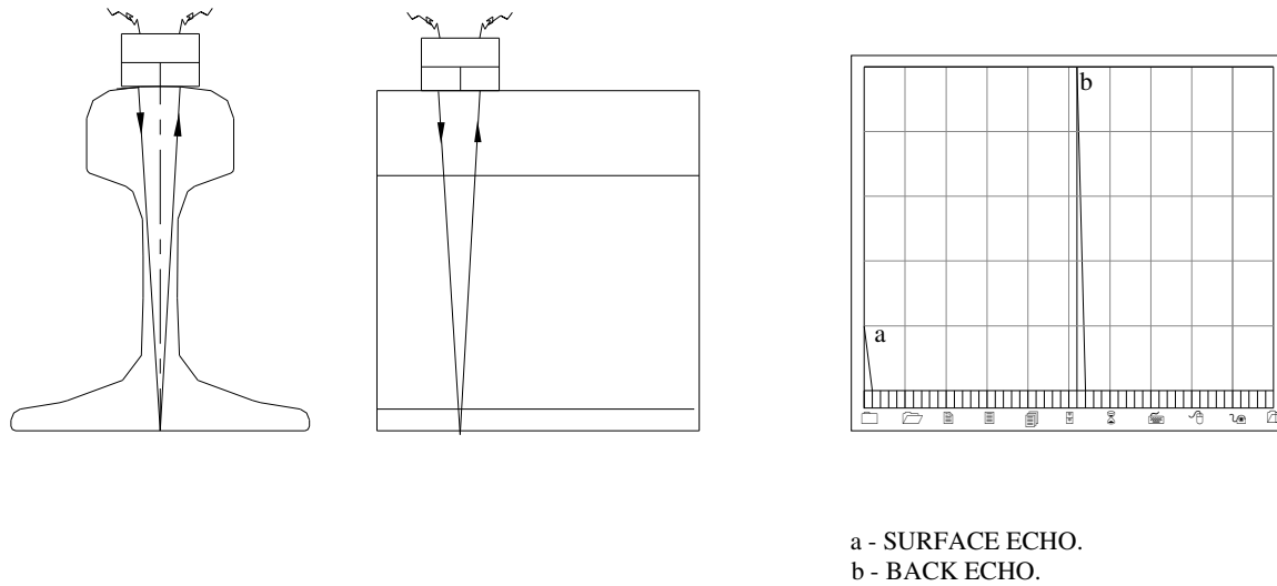
FIG.5: RAIL WITHOUT FLAW (0° PROBE)
