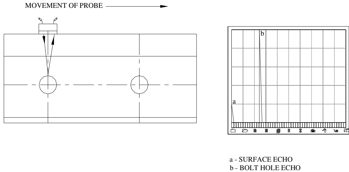
FIG. 15 : BOLT HOLE WITHOUT CRACK (0° PROBE)
