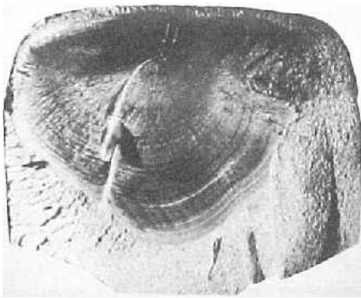
FIG. 50 : 411 - WELDING, FLASH BUTT JOINT, TRANSVERSE CRACK
