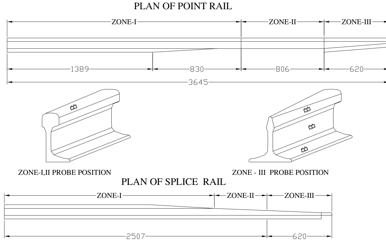
FIG. 26(a): TESTING PROCEDURE FOR POINT AND SPLICE RAILS FOR 1 IN 12 CROSSING B G 52 Kg
