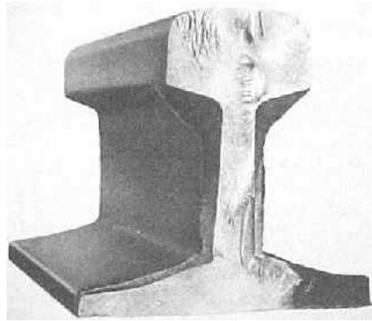
FIG. 50 : 411 - WELDING, FLASH BUTT JOINT, TRANSVERSE CRACK
