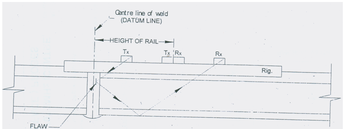
Fig. 22(c) : AT weld testing using 45^\circ tandem probe
