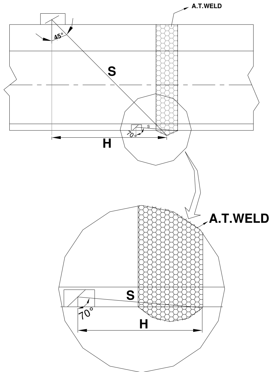
FIG. 21(b): TESTING OF BOTTOM FLANGE OF A.T. WELDS USING 70^\circ AND 45^\circ PROBES
