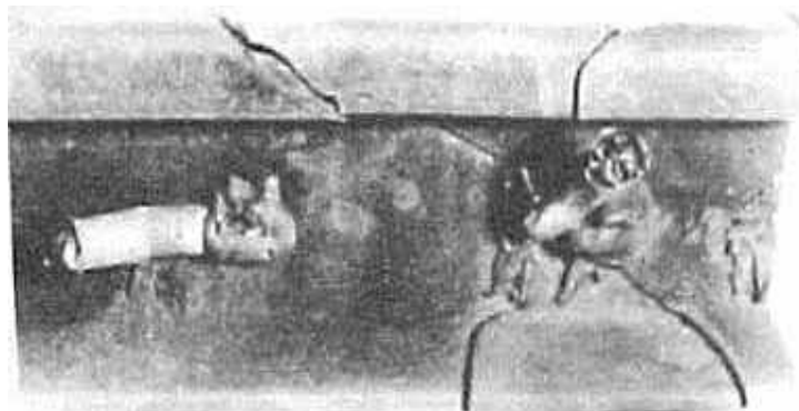
FIG. 56 : 481 - WELDING, TRACTION BOND WELDING CRACK AT WELD
